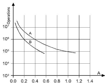
Contact loading: 110Vdc, L/R 40 ms Curve A: RMM.x6-7-8 Curve B: RMM.x2-3-4
