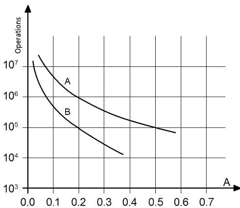
Contact loading: 110Vdc, L/R 40 ms Curve A: RMMZ11 Curve B: RGMV12-13, RMMV12-13
