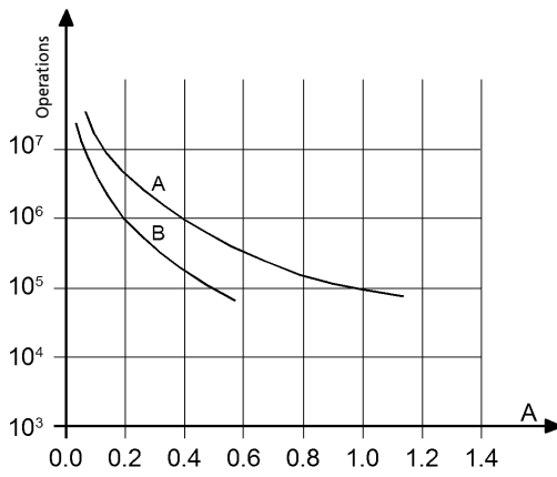
Contact loading: 110Vdc, L/R 40 ms Curve A: RMN_xy Curve B: RMD_xy
