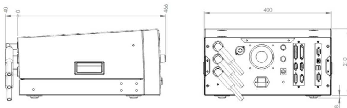
Housing dimensions with angled plugs:
