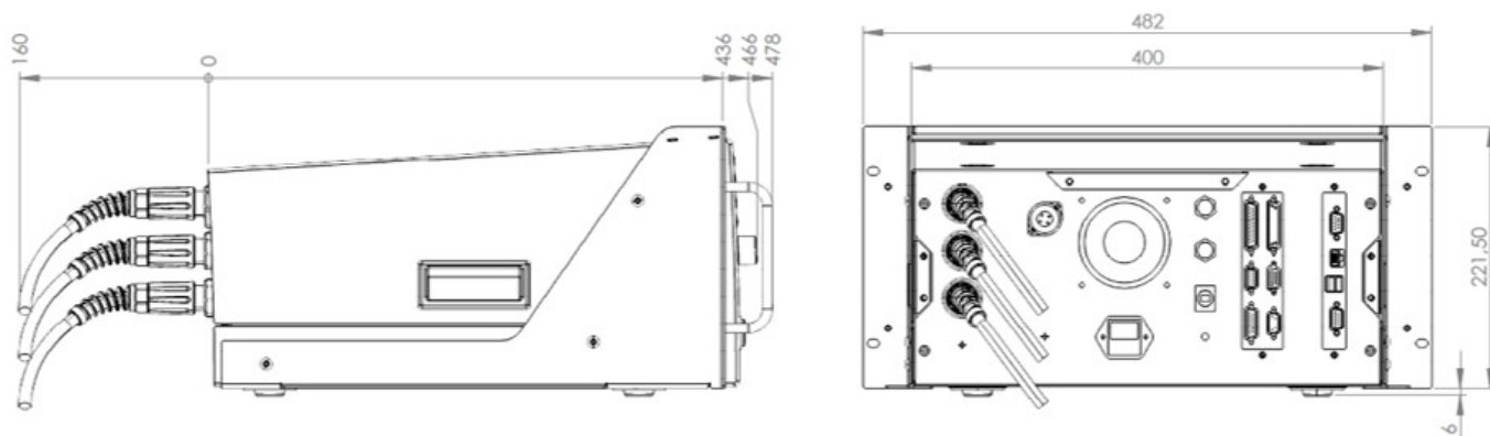
Housing dimensions with installation set 19 inches:
