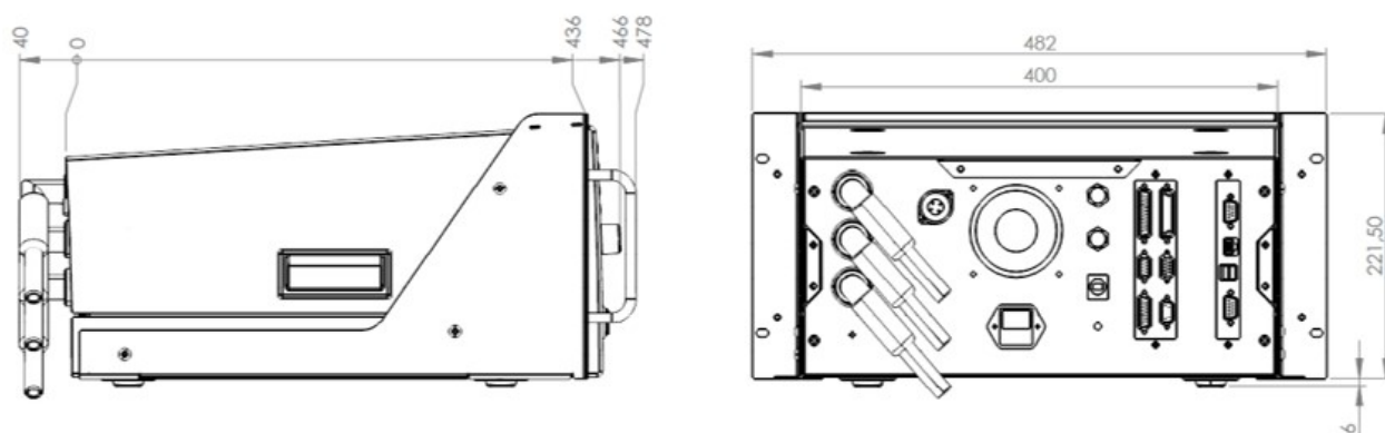
Housing dimensions with installation set 19 inches and angled plugs:
