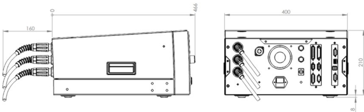
Housing dimensions with angled plugs:
