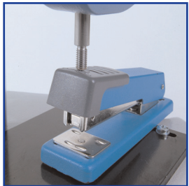
Actuation testing
