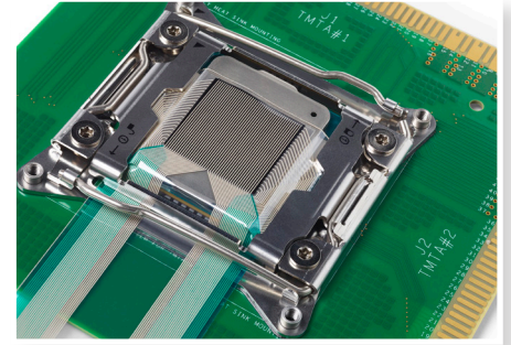
Heat Sink with Pressure Mapping Sensor
