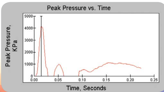
Peak pressure vs. Time graph showing force on a crash test dummy knee
